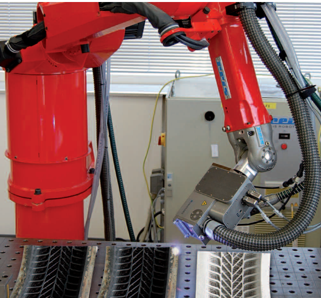
Robot guided laser system
