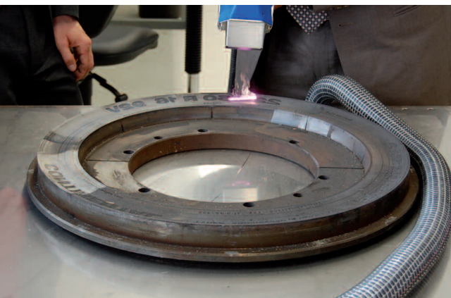
Handheld Manually Operated Laser Cleaning
